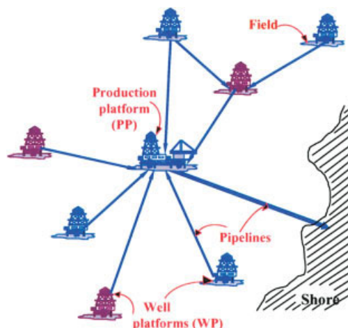
Figure 9. Infrastructure for off-shore gas production.
