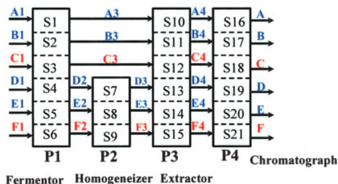
Figure 7. Multistage batch plant for protein manufacturing.
