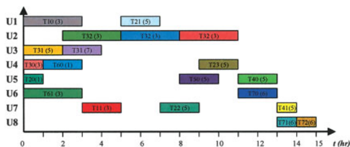
Figure 12. Optimal schedule with makespan of 15 hours.
