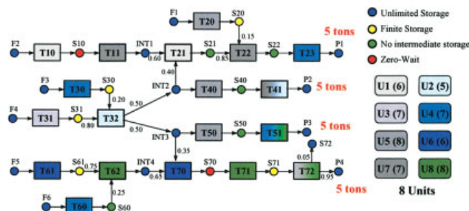
Figure 11. State-task network for batch process manufacturing products P1, P2, P3, P4.
